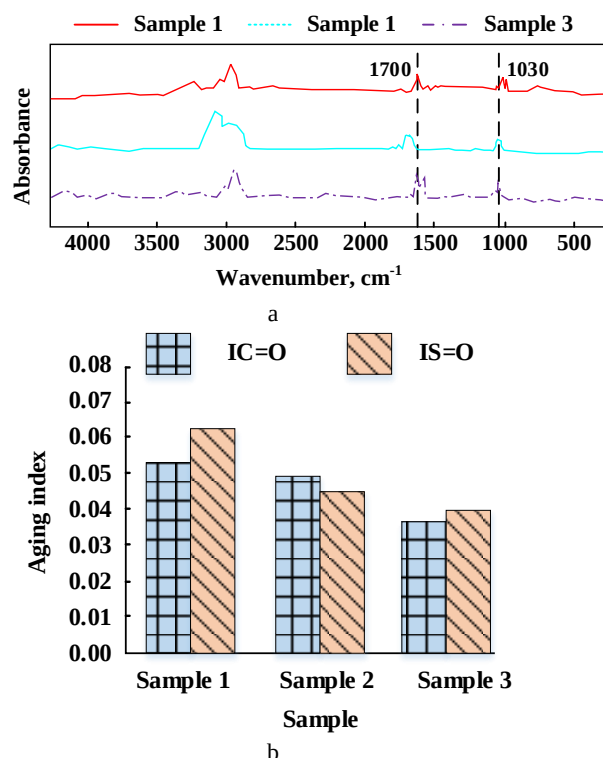
Fig. 8. FTIR and aging indices of carbonyl and sulfoxide groups for three asphalt samples: a–FTIR; b–aging index of carbonyl and sulfoxide groups
