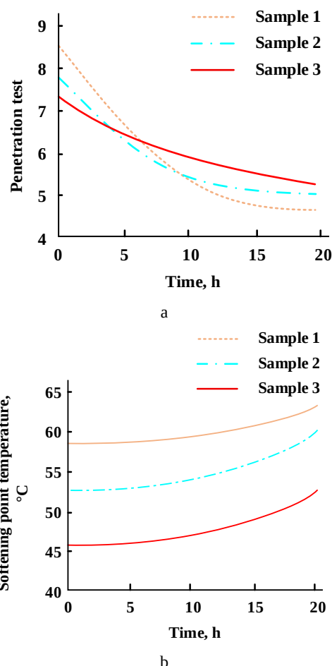
Fig. 7. Penetration and softening point tests of three asphalt samples: a–penetration test; b–softening point test
