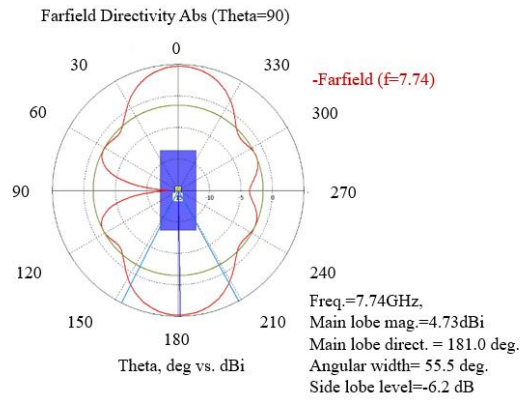
Fig. 7. Far-field and near-field from CST Studio Suite zinc tungstate-5 wt.% B 2 O 3 -epoxy composite: a – 3D radiation pattern shows the total realized gain of the microstrip antenna at 7.74 GHz; b – geometric configuration and design parameters of microstrip antenna; c – radiation pattern depicted in cartesian coordinates at resonance frequency; d – polar radiation pattern (E plane and H plane) of microstrip antenna at 7.74 GHz; e – surface current distribution on microstrip antenna at resonance frequency
