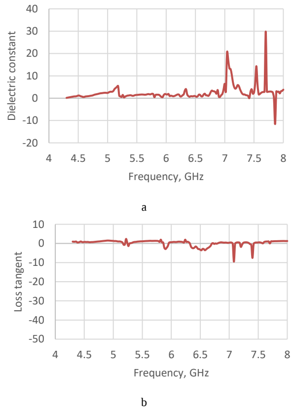
Fig. 2. Dielectric properties of zinc tungstate with boron oxide (5 %) composite at frequency rang 4–8 GHz: a – dielectric constant of zinc tungstate with boron oxide (5 %) composite; b–loss tangent of zinc tungstate with boron oxide (5 %) composite
