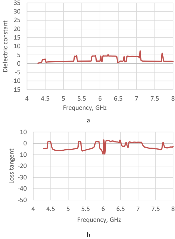
Fig. 3. Dielectric properties of zinc tungstate (5 %) composite at frequency rang 4–8 GHz: a–dielectric constant of zinc tungstate (5 %) composite; b–loss tangent of zinc tungstate (5 %) composite
